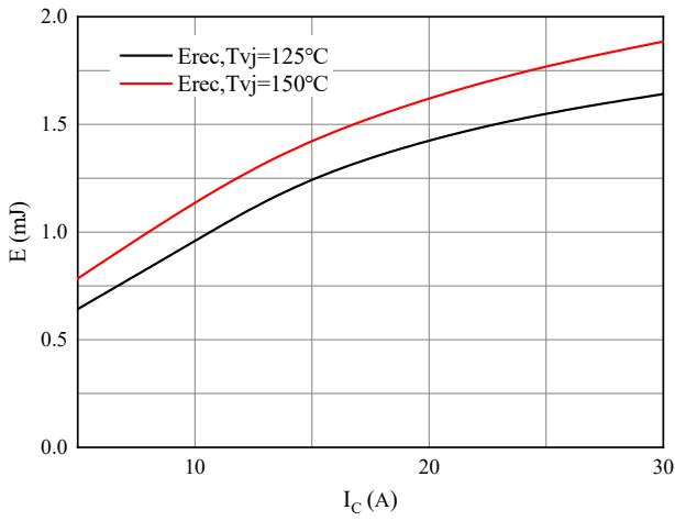
Figure 5. Switching losses of IGBT VGE=±15V, RGon=40Ω, RGoff=40Ω, VCE=600V
