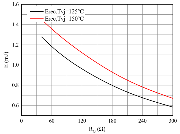
Figure 6. Switching losses of IGBT VGE=±15V, IC=15A, VCE=600V
