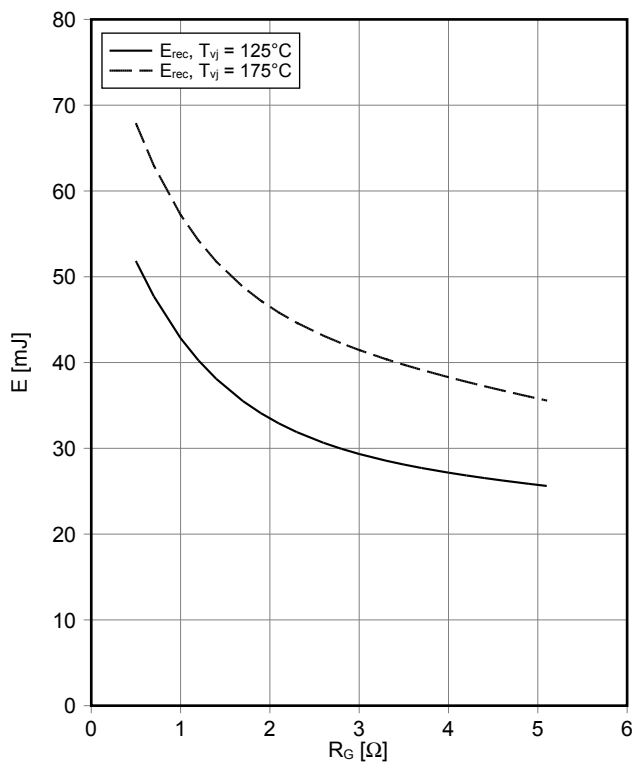
开关损耗 二极管,逆变器 (典型) switching losses Diode, Inverter (typical) E_{rec} = f(R_G) I_F = 900 \text{ A}, V_{CE} = 600 \text{ V}
