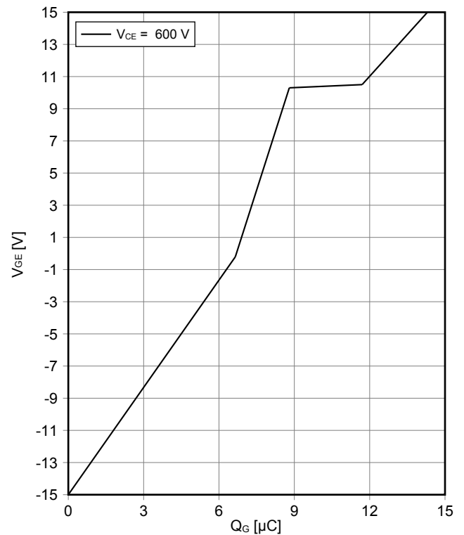
栅极电荷特性 IGBT, 逆变器 (典型) gate charge characteristic IGBT, Inverter (typical) V_{GE} = f(Q_G) I_C = 900 A, T_{vj} = 25^\circ C
