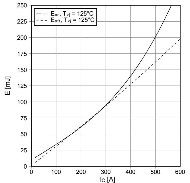
Schaltverluste IGBT-Wechselr. (typisch) switching losses IGBT-inverter (typical) E_{on} = f(I_c), E_{off} = f(I_c) V_{GE} = \pm 15\text{ V}, R_{Gon} = 4.7\ \Omega, R_{Goff} = 4.7\ \Omega, V_{CE} = 900\text{ V}
